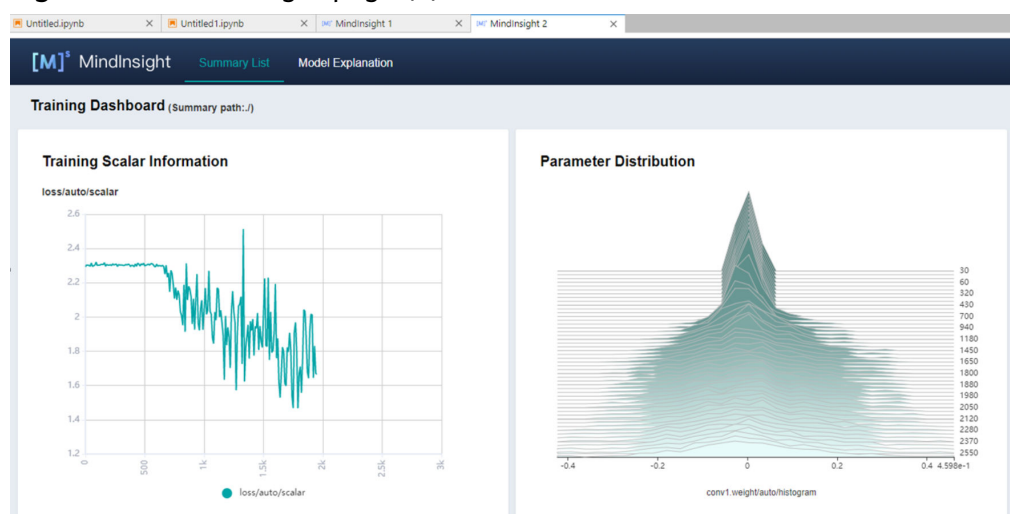
Figure 4-37 MindInsight page (3)
