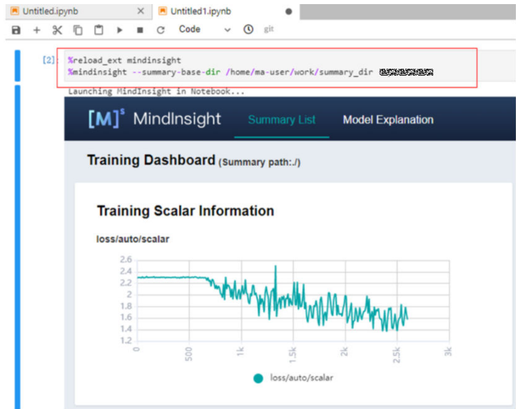
Figure 4-33 MindInsight page (1)
