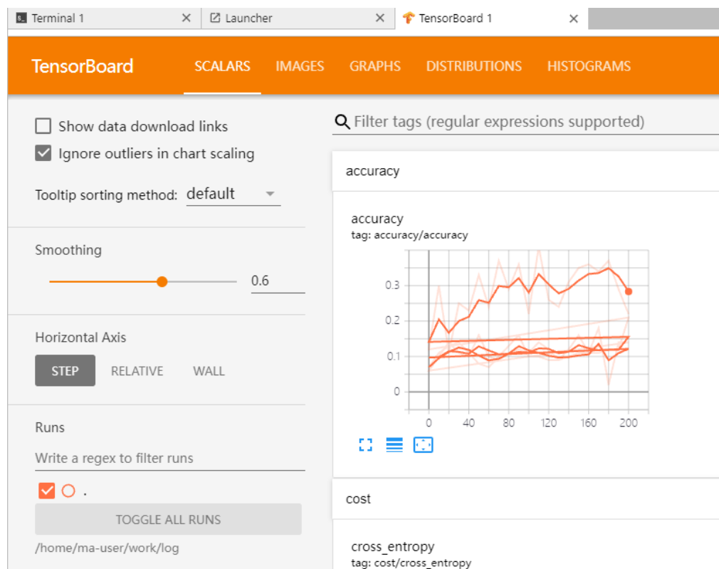
Figure 4-46 TensorBoard page (3)
