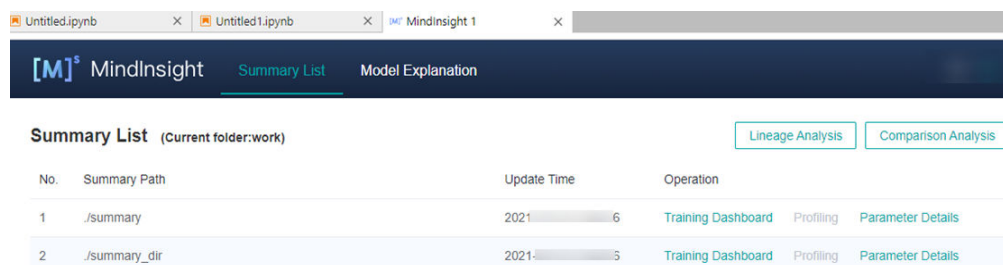
Figure 4-34 MindInsight page (2)
